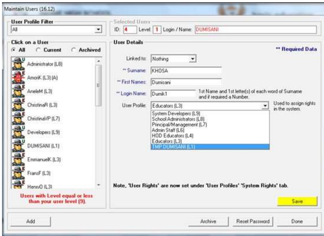
Figure 17: Maintain Users
