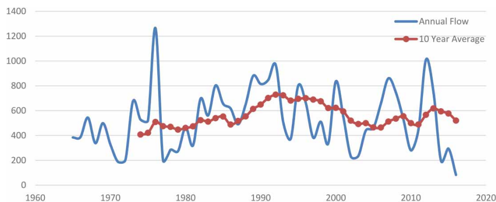
Figure 7 | Changes in the annual and ten-year moving average for flow (Mm 3 /a) in the Berg River at G1H013.
