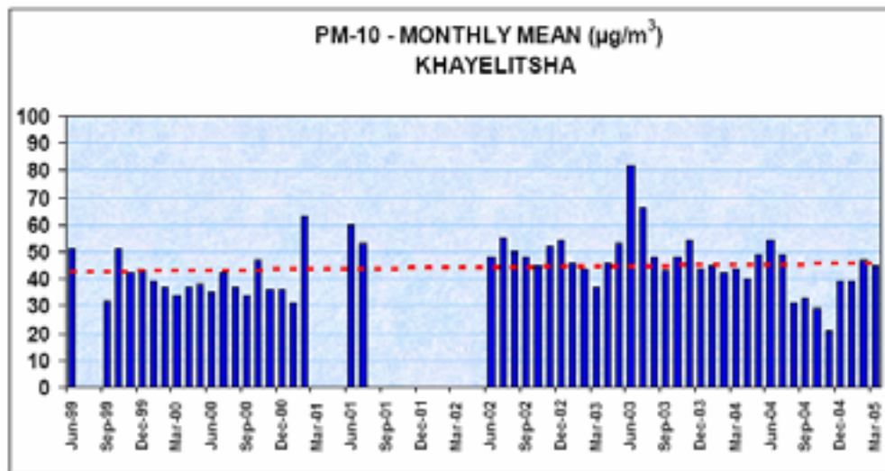
Figure 16: Monthly mean PM10 values at Khayelitsha
