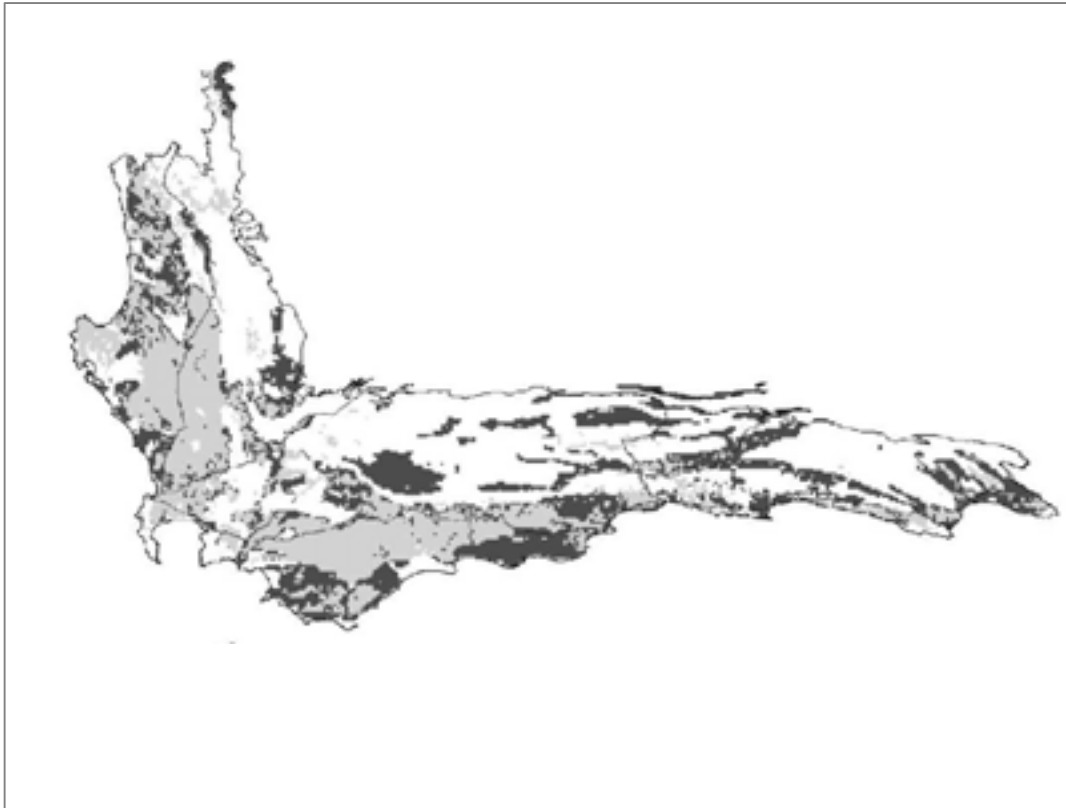
Figure 3: Current (light grey) and projected distribution within 20 years (dark grey) of land transformed by agriculture and forestry in the Cape Floristic Region (Rouget et al. 2003).
