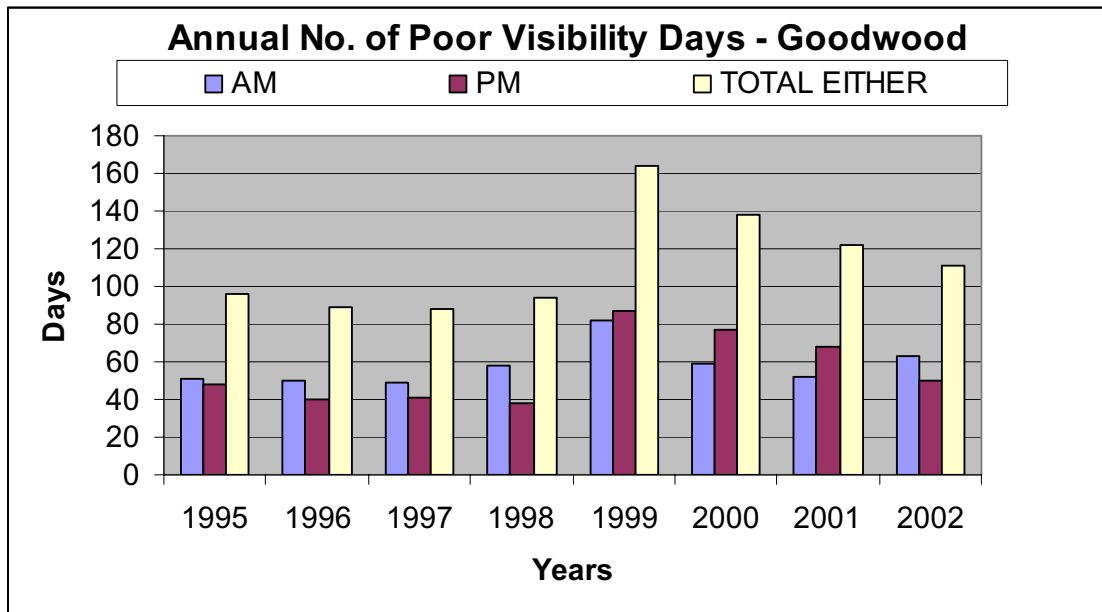
Figure 15: Annual number of poor visibility days - Goodwood
