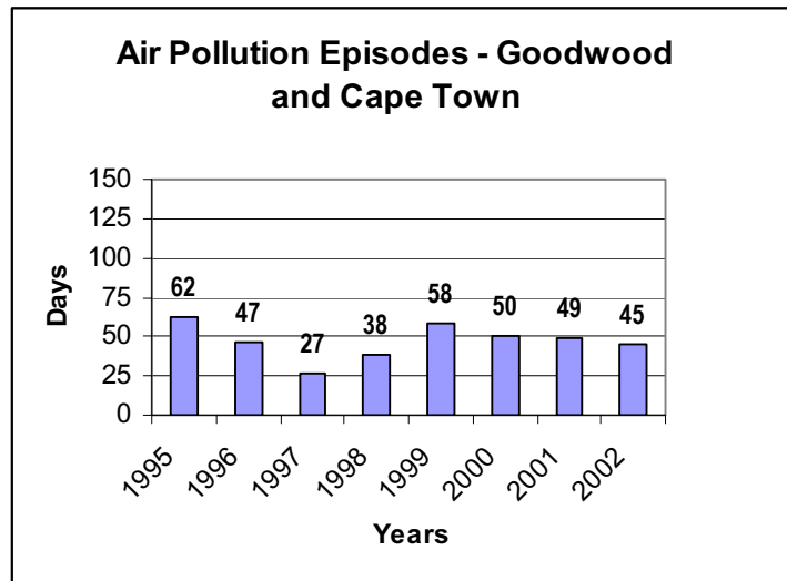
Figure 14: Annual number of Air Pollution events - Cape Town city Centre and Goodwood
