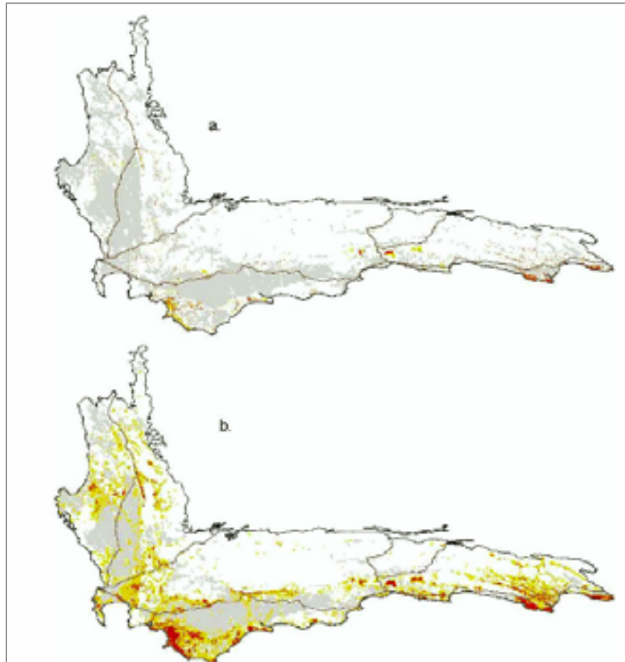
Figure 4: Current (a) and projected distribution within 20 years (b) of land transformed by alien plant infestation (lightly invaded in orange, densely invaded in red) in the Cape Floristic Region (Rouget et al. 2003). Current transformation by agriculture is shown in grey.
