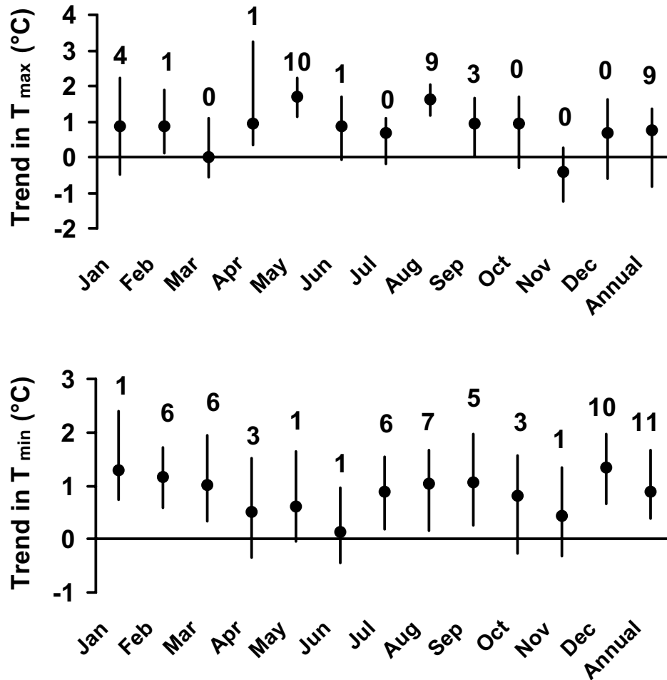
Figure 6: Trends in minimum ( T_{min} ) and maximum ( T_{max} ) monthly temperatures (January to December from left to right on the X-axis, followed by the annual mean), for 12 Western Cape climate stations during the last three to four decades of the 20th century. The filled circles represent mean change for all stations, and the bar represents the range between lowest and highest trend value. The number above each data entry represents the number of stations out of twelve for which the linear change is statistically significant (>95% confidence level). Trends in maximum temperatures are consistently highest in spring and autumn, while minimum temperature trends are high all year round, but particularly so in summer months.
