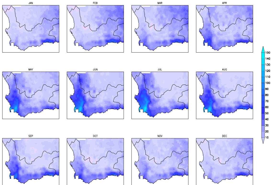
Figure 7: Climatological monthly precipitation totals (mm)
