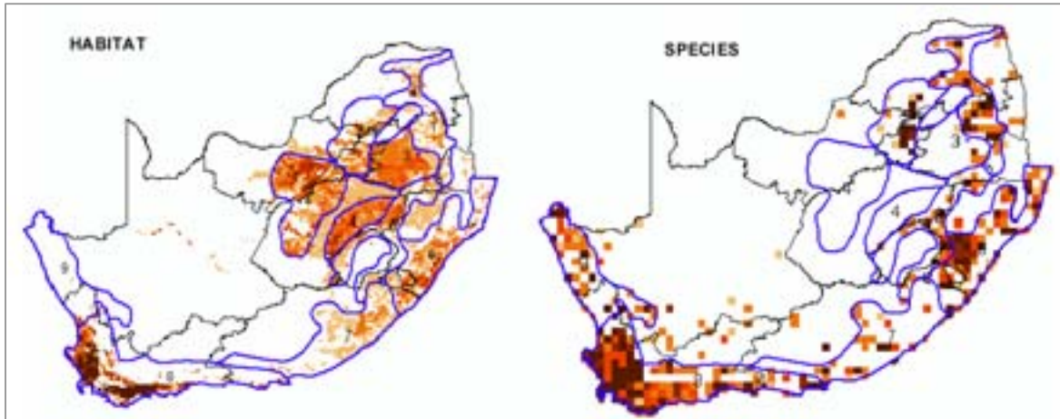
Figure 2: Indices of irreplaceability for habitats (left hand panel) and species (right hand panel) with darker colours indicating higher irreplaceability. Irreplaceability is an index of rarity and uniqueness. The Western Cape clearly shows an extreme concentration of irreplaceable habitats and species in relation to the rest of South Africa (Figure from Driver et al. (2005)).
