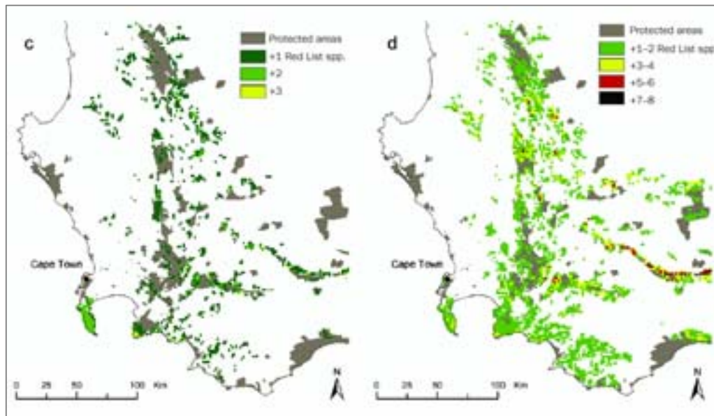
Figure 13: Projected change, by ~2020, in the number of threatened Protea species found in the current protected area network in the Western Cape under two different scenarios: Change in red-listed species induced by land transformation alone (left hand panel) and the change in red listed species induced by a combination of land transformation and climate change (right hand panel). Climate change impacts will therefore place a greater burden on the current protected areas system, will increase the importance of this network in conserving endemic species, and will create a need to increase the size of the protected area system.
