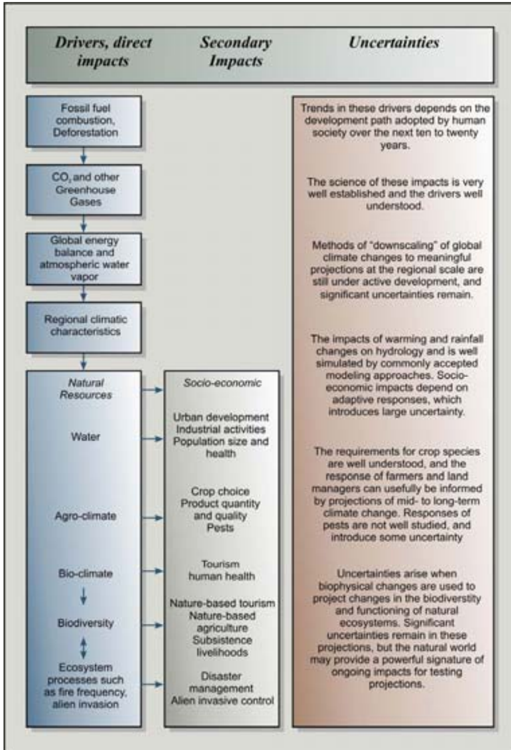
Box 2: Key drivers of climate change, their direct and secondary impacts, and the uncertainties associated with them
