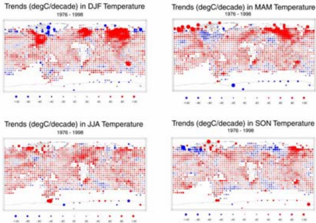
Figure 5: Historical trend in seasonal mean temperature (from IPCC, 2001b)
