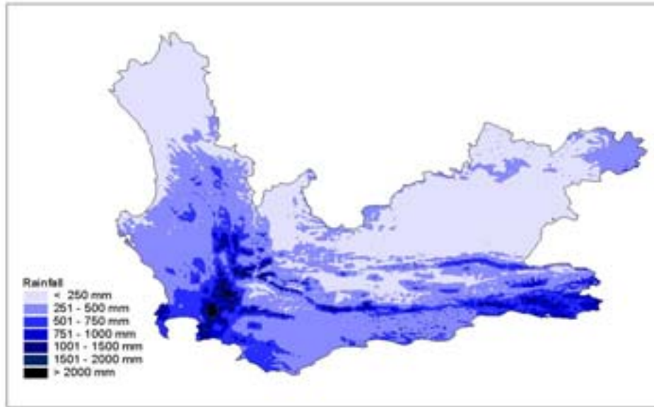
Figure 1: Mean annual rainfall of the Western Cape
