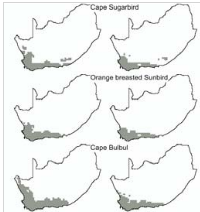
Figure 12: Current (left hand column) and future (right hand column) modeled geographic ranges for three Cape bird species, according to a climate scenario for ~2050 (from Simmons et al. 2005)
