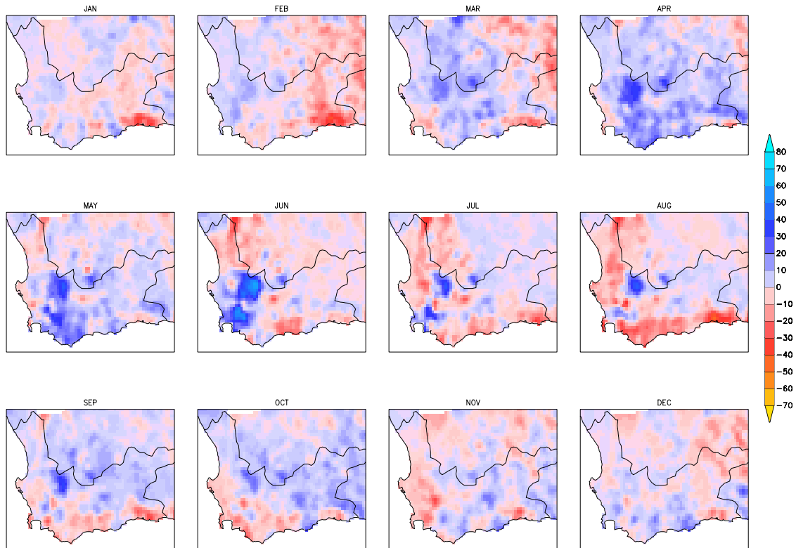
Figure 8: Trend in monthly total precipitation (mm) for 1950-1999 (as the total change in mm over 50 years), red tones represent drying, and blue tones wetting trends.
