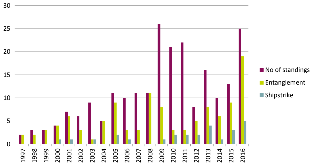
Figure 1: Number and type of marine mammal strandings (1997-2016)
