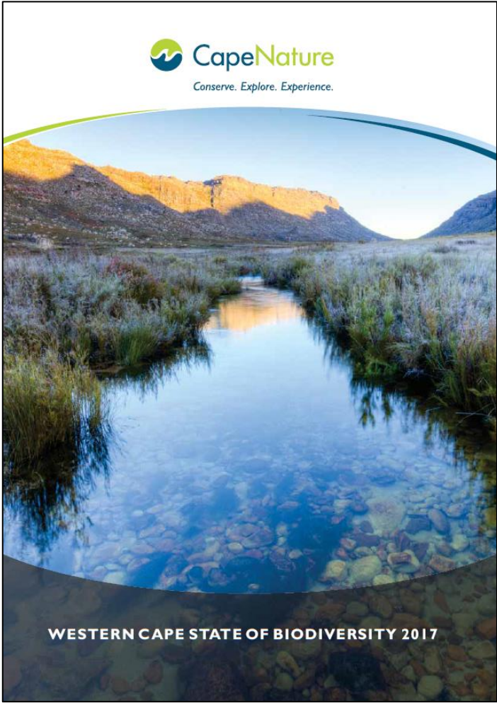
Figure 3: Western Cape State of Biodiversity Report (2017)
