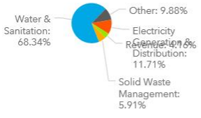
I faults
